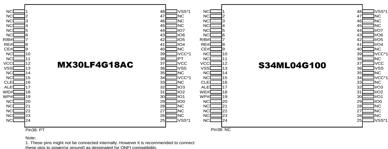
Figure 5-1: 48-TSOP (12x20mm) Package and Pin Layout Comparison
