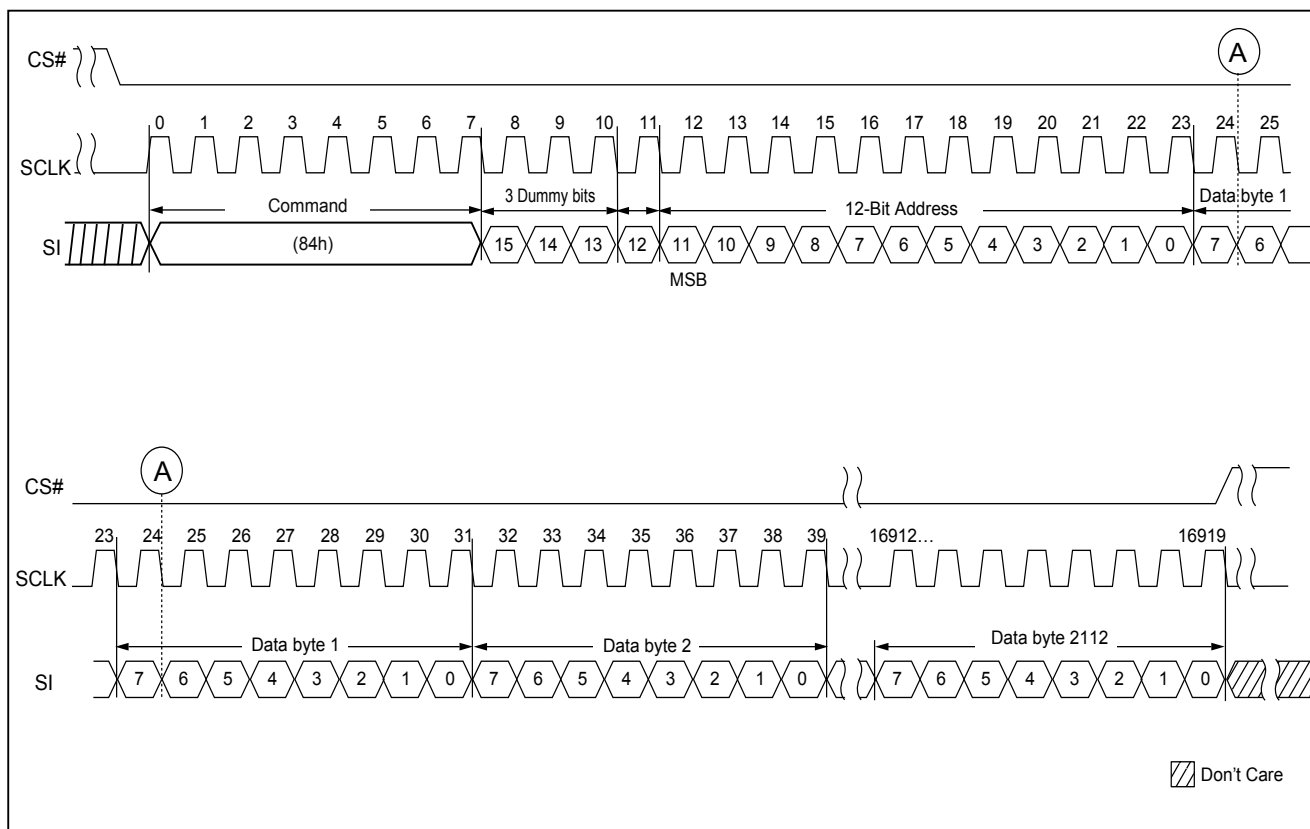
Figure 19. PROGRAM LOAD RANDOM DATA (84h) Timing
