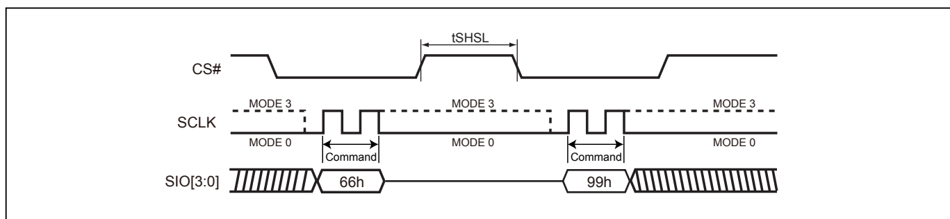
Figure 109. Reset Sequence (QPI mode)
