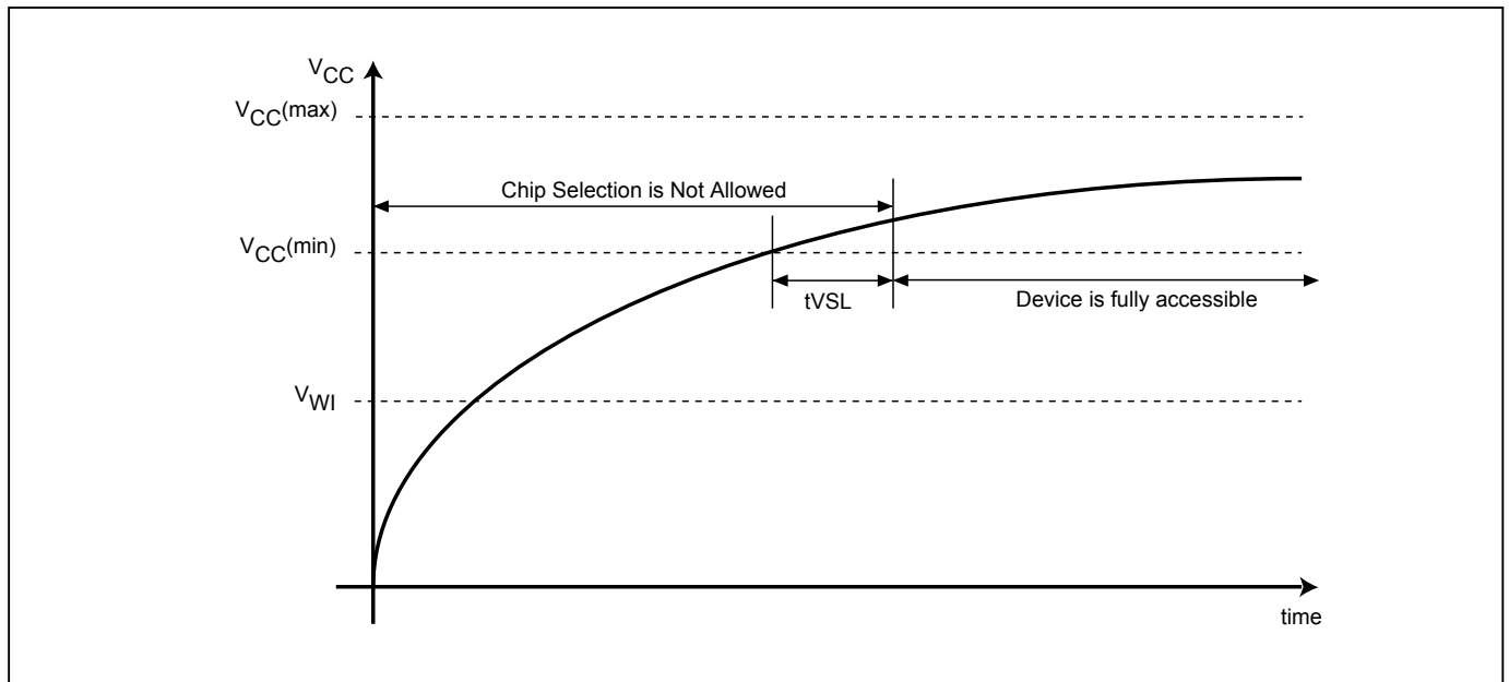
Figure 38. Power-up Timing
