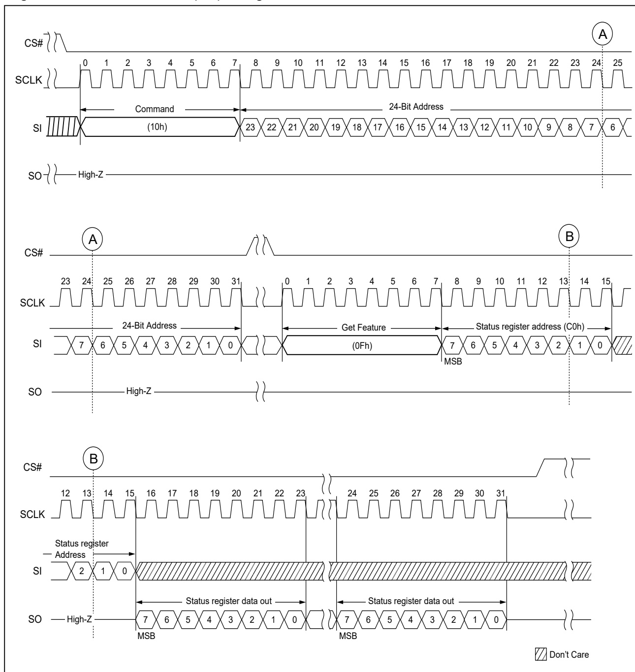
Figure 26. PROGRAM EXECUTE (10h) Timing
