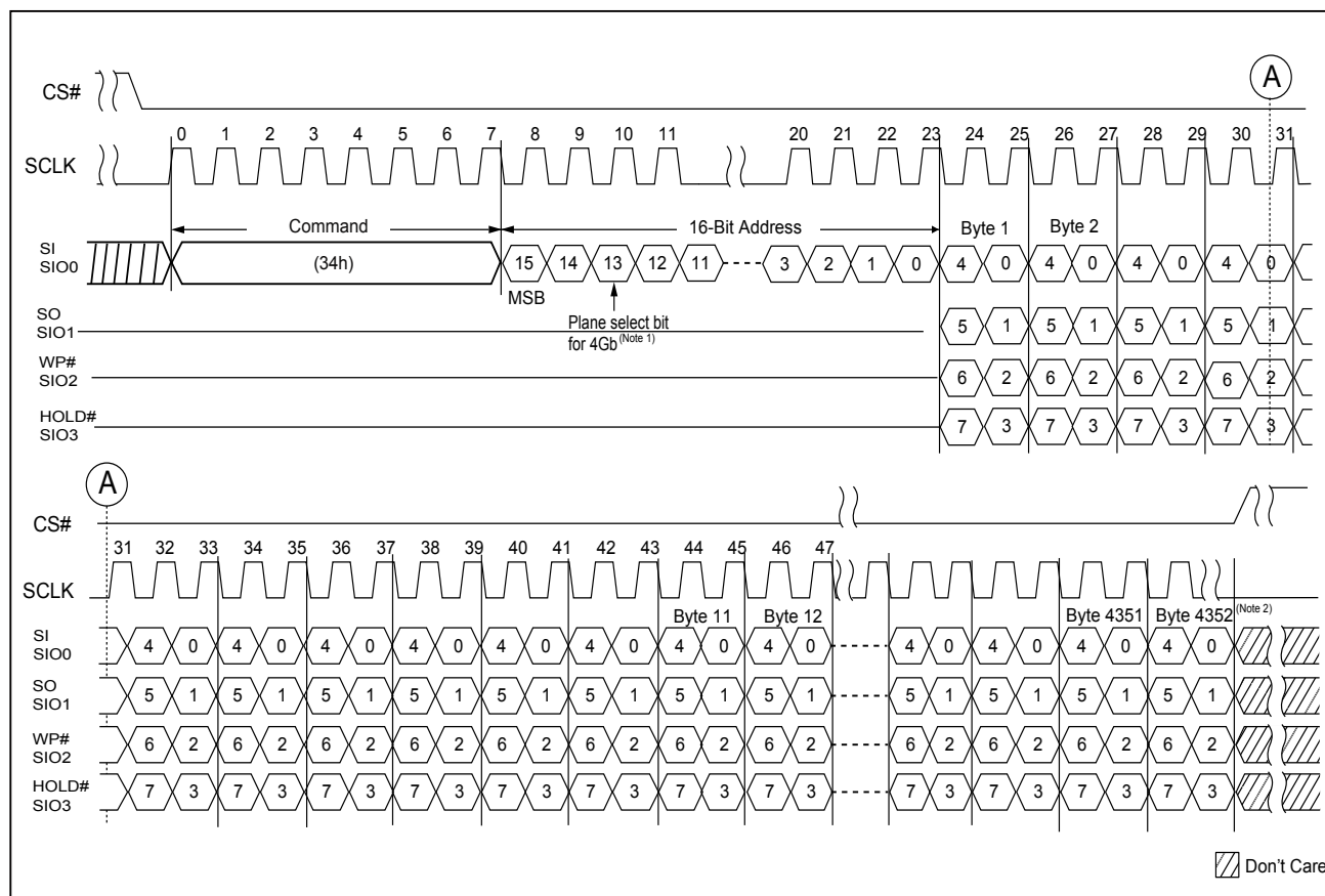
Figure 25. QUAD IO PROGRAM RANDOM INPUT (34h) Timing
