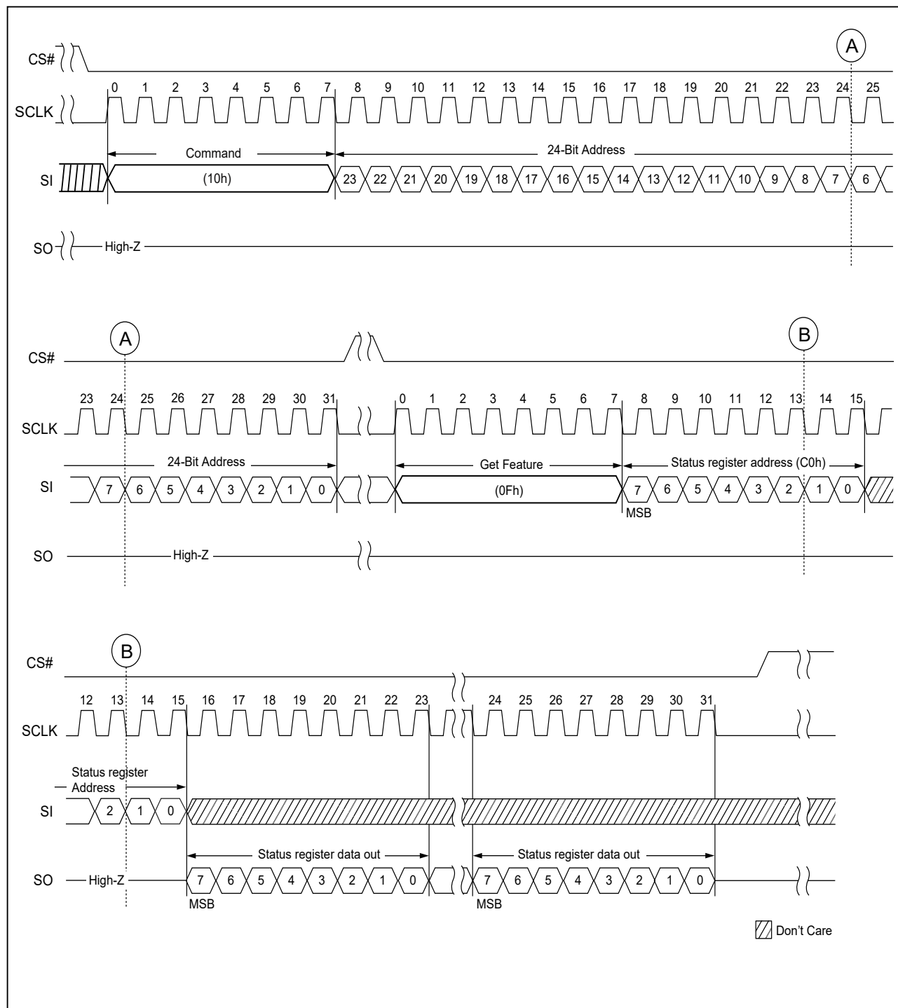
Figure 27. PROGRAM EXECUTE (10h) Timing
