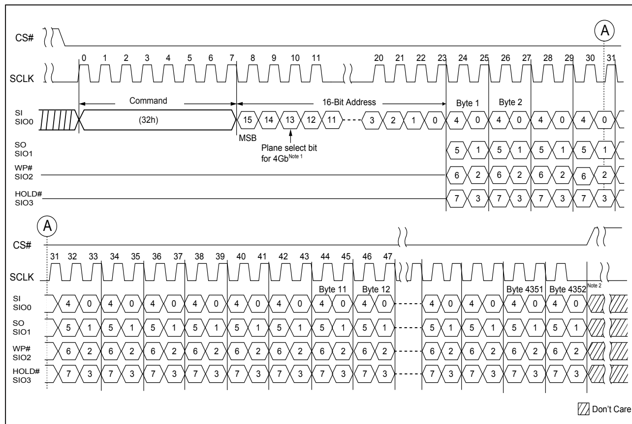
Figure 25. PROGRAM LOAD X4 (32h) Timing
