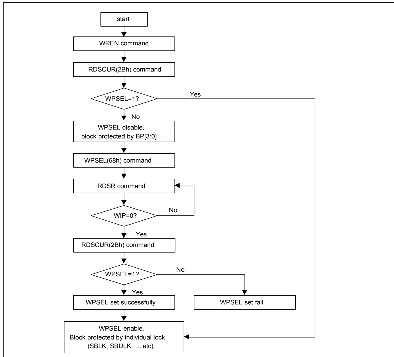
Figure 73. WPSEL Flow
