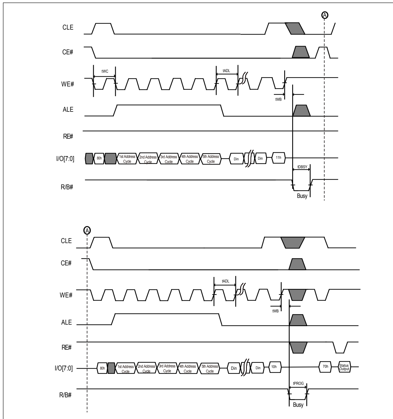
Figure 38-1. AC Waveform for Two-plane Program (ONFI)
