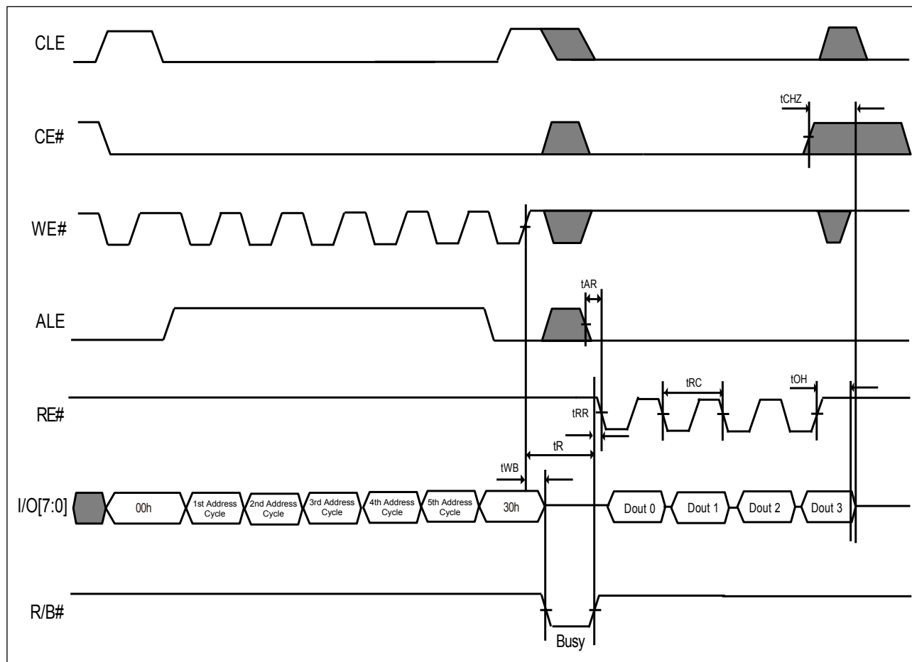
Figure 7. AC Waveforms for Read Operation (Intercepted by CE#)
