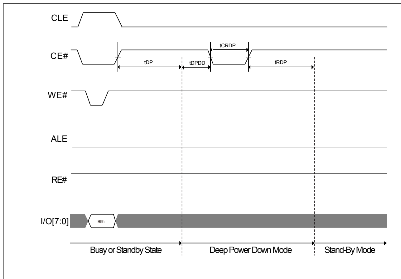
Figure 23. AC Waveform for Deep Power-down Mode operation
